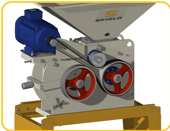
Grooved cast-iron pulley
